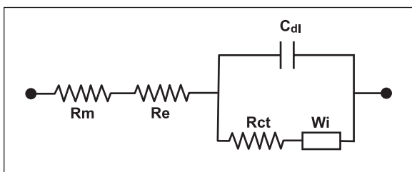
Figure 6 Randles equivalent circuit
