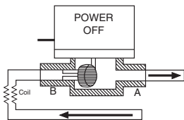
Figure-3a 2-Way Valve With Normally Closed Actuator.
