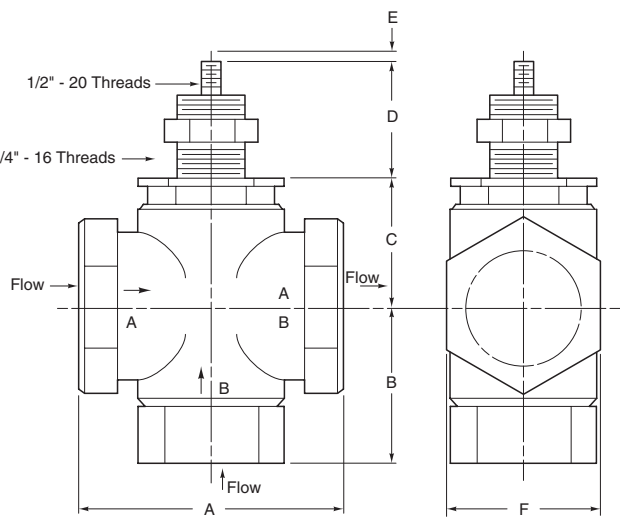
Figure 9. Typical of VB-9313-0-4-P, 2½" and 3" Valve Bodies.
