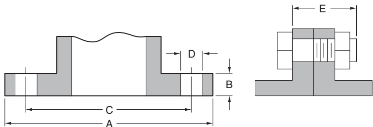
Figure 11. Flange Dimensions.
