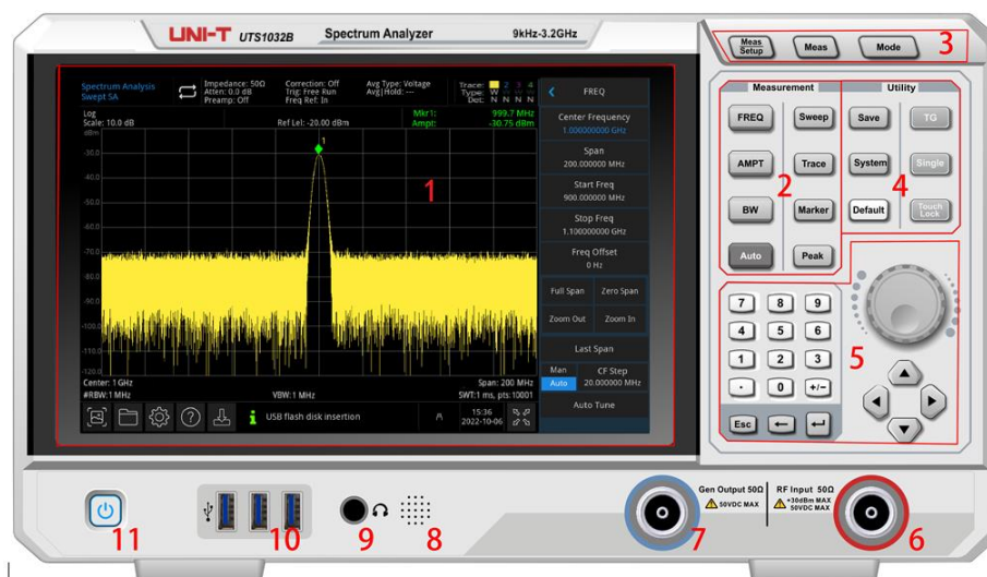
Figure 1-1 Front Panel
