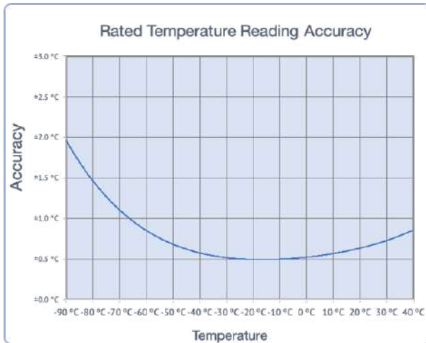
Figure 4: Rated Temperature Accuracy Chart
