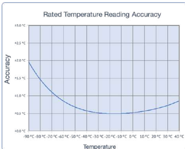
Figure 6: Rated Temperature Accuracy Chart
