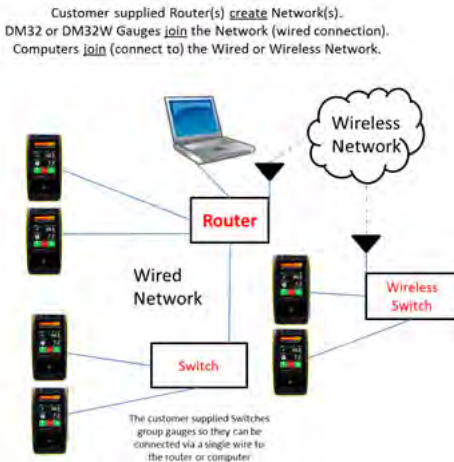
Figure 57: Multiple gauge connection and networking possibilities with the DM32
