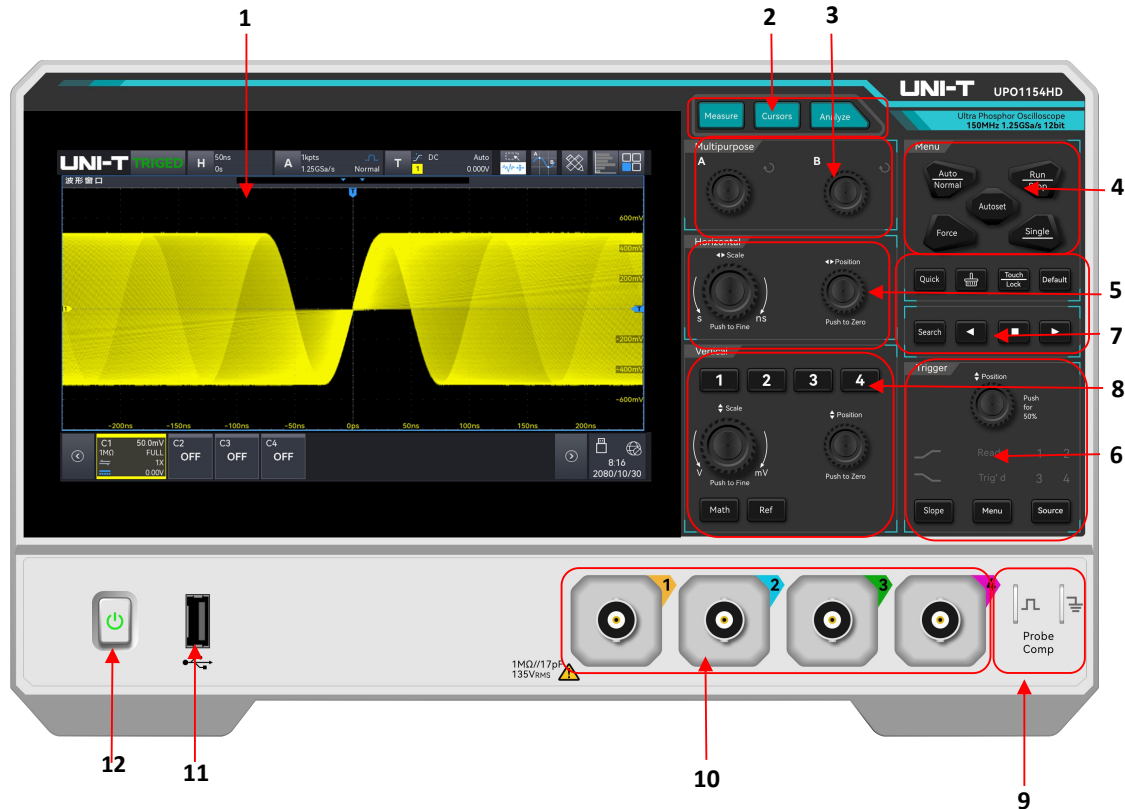
Front Panel
