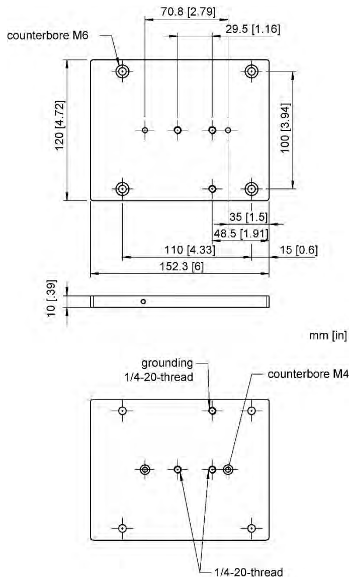
Figure 7-20: Mounting Base
