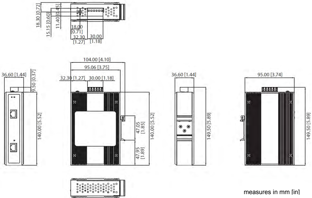
Figure 7-14: Dimensions
