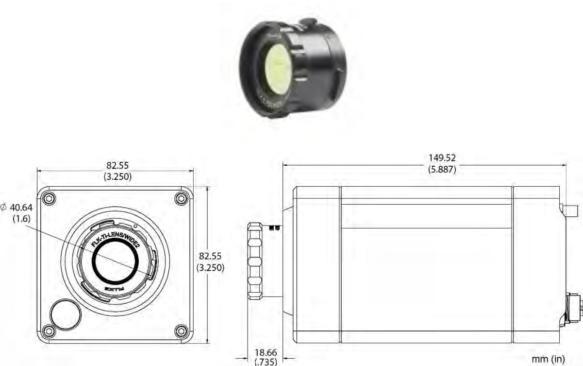
Figure 7-1: Wide Lens
