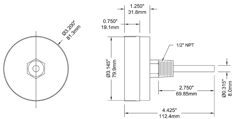
3" Back Connection
