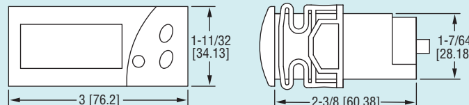
Panel Cutout 2-51/64" x 1-9/64" (71 x 29 mm)
