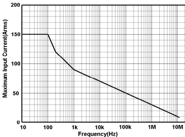
T3CP150-12 Continuous Maximum Current Input
