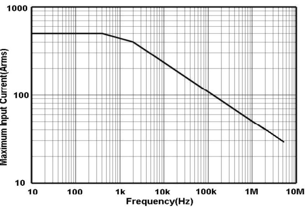
T3CP500-5 Continuous Maximum Current Input
