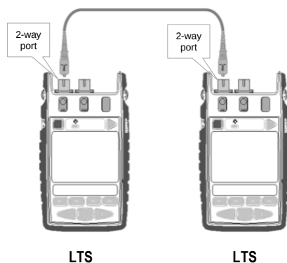
Figure 15A. Test set up for length measurement referencing
