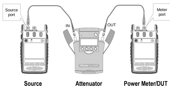
Figure 8. Test set-up for the Power Meter section Accuracy Test
