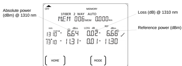
Figure 4. Memory display of Two-Way Autotest (Test summary)
