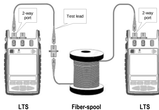
Figure 15B. Test set up for length measurement accuracy verification
