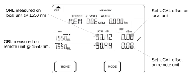
Figure 6. Memory display of Two-Way Autotest (ORL test)
