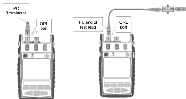
Figure 16A. Test set up for ORL verification test
