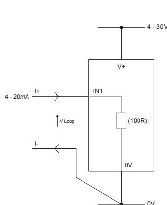
MEASURING 4-20mA
