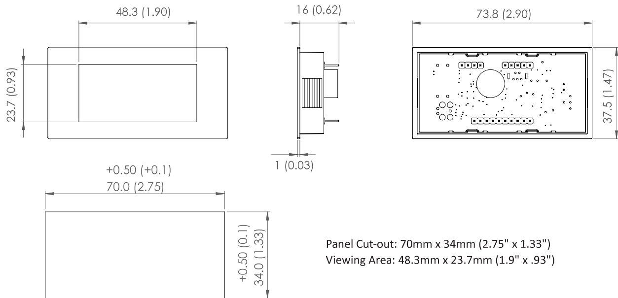
Panel Cutout
