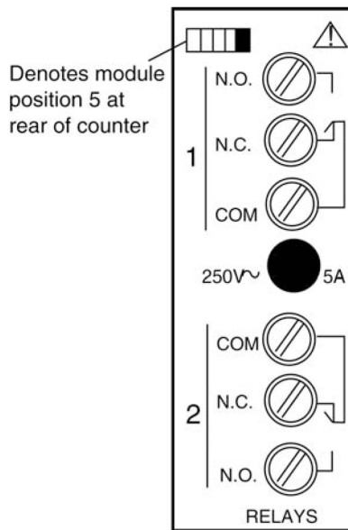
Figure 15. Dual Relay
