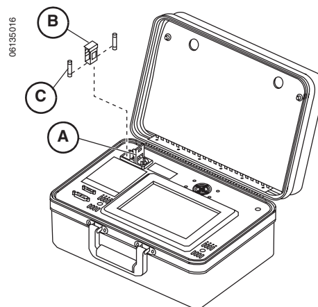
Figure 73: Fuse Replacement
