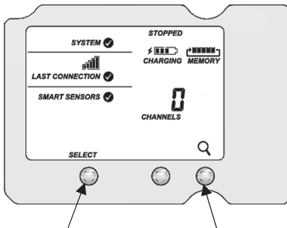
Press the Select button to view the smart sensor screen
