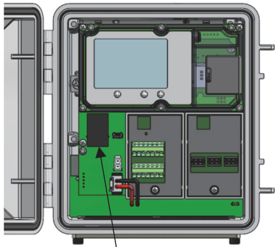
Plug in an Ethernet cable here
