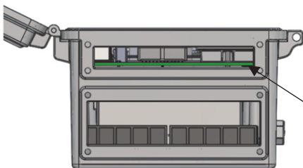
Feed analog sensor and relay cables through this opening to connect them to the optional modules
