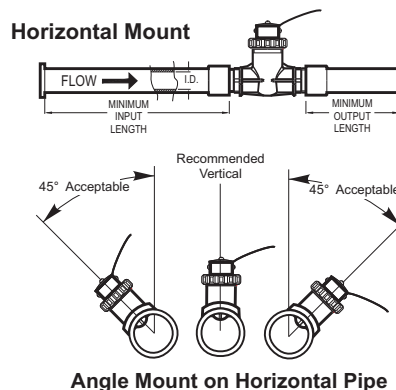
Angle Mount on Horizontal Pipe
