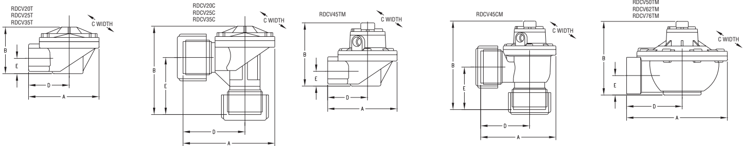
RDCV Dimensional Chart
