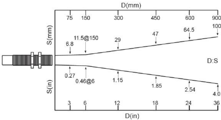
Figure 1 : Optical diagram
