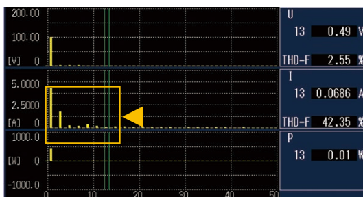
THD and dominant orders
