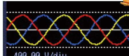
Waveform as measured by the PW3365
