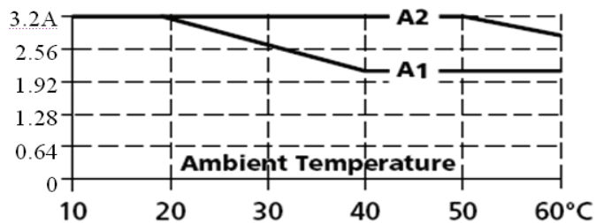
Output Current
