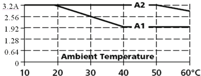
Output Current
