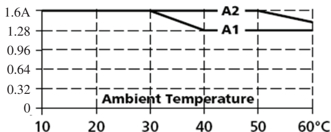
Output Current
