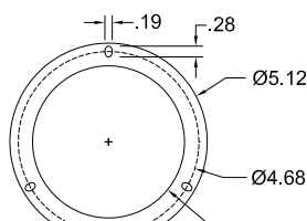
4" MOUNTING FLANGE
