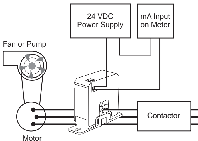
Figure 1: Measuring Current Using PDA6420 Current Transducer
