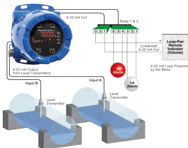
Round Horizontal Tank Signal Input Conditioner
