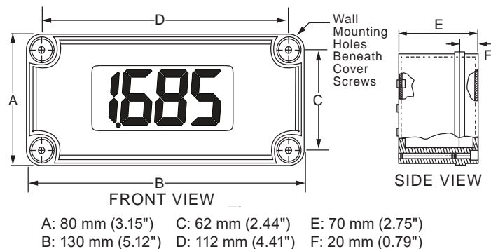
Figure 7: Dimensions and Wall Mounting Information
