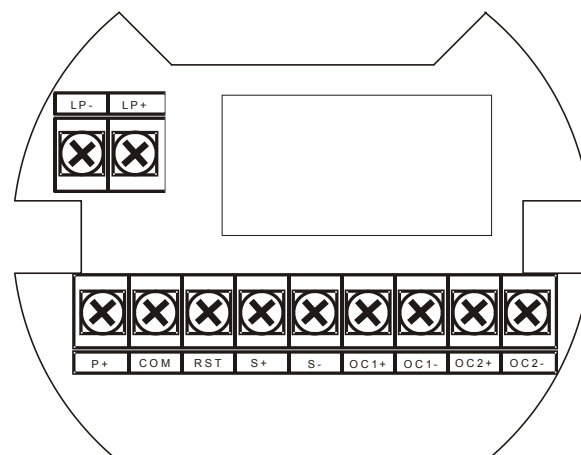
Figure 1. Connector Board
