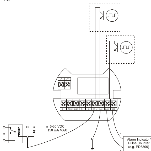
Figure 13. Open Collector Output Connections
