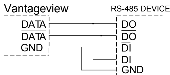
Figure 12. RS-485 4 Wire Serial Connections
