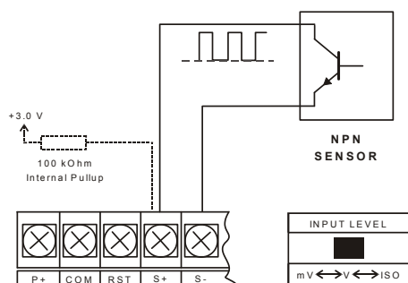
Figure 5. NPN Open Collector Input (NPN)
