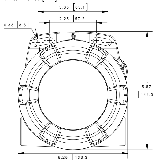
Figure 16. Enclosure Dimensions – Front View
