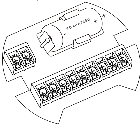
Figure 14. Battery Orientation
