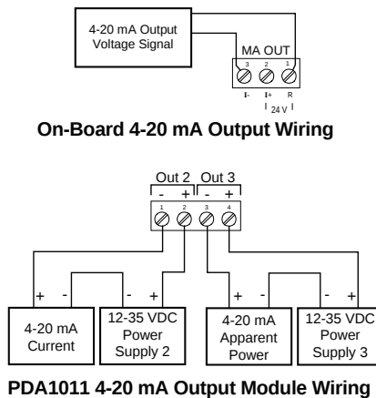
PDA1011 4-20 mA Output Module Wiring
