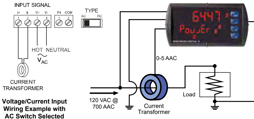
Voltage/Current Input Application Example
