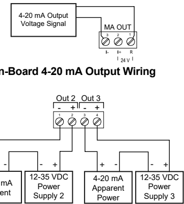
PDA1011 4-20 mA Output Module Wiring
