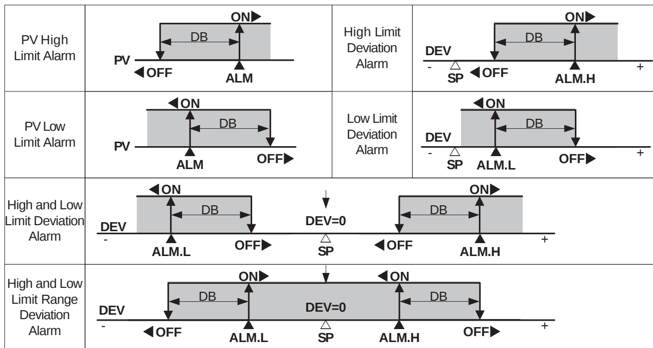
Fig 6: Alarm Operation
