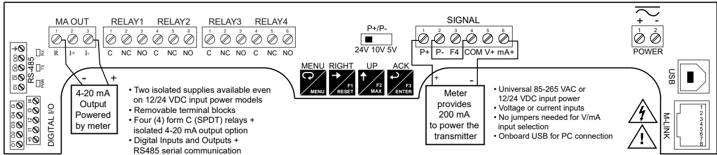
Connector Labeling for Fully Loaded PD2-6000
