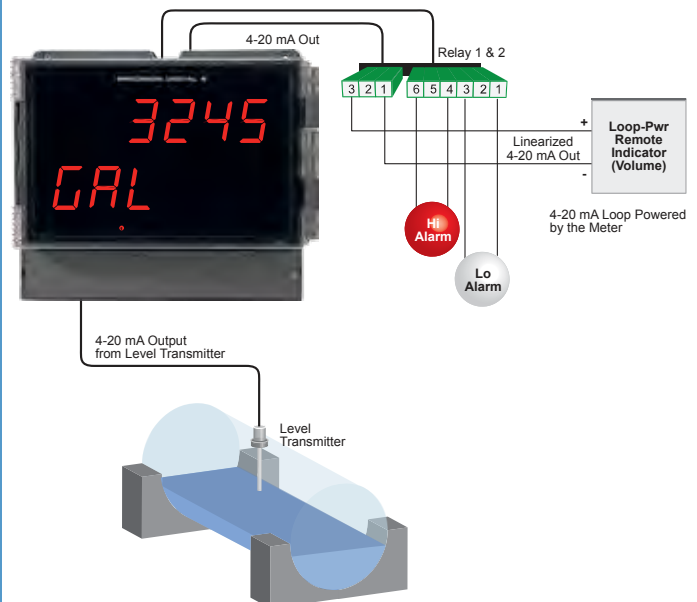
Round Horizontal Tank Signal Input Conditioner
