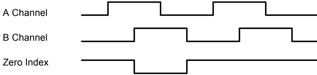
Allen Bradley: current source, CCW rotation.
