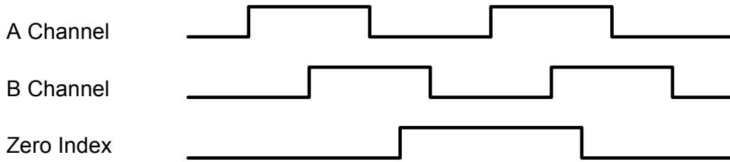
Allen Bradley: current sink, open collector & line driver, CCW rotation
