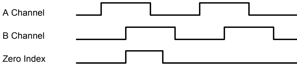
BEI: Models MX-51, MX-21, CCW rotation
