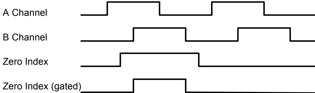
BEI: Models H25, L25, E25, MOD5500, MOD5600, CCW rotation
