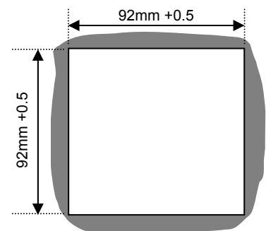
Cut-out
