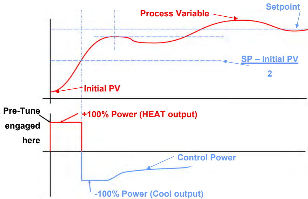
Figure 44. Pre-Tune Operation
