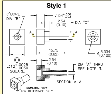
Crimp Style Brass or SS Bushing also available
