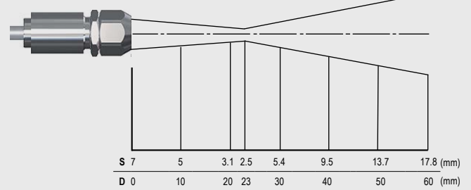
Optics CT LT CF, D:S = 2:1 (far field = 2.5:1)
