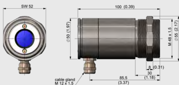
Sensing head
