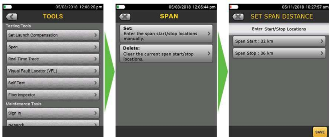
Process to set Span on an OptiFiber Pro OTDR
