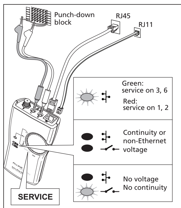
Figure 3. Validating Ethernet Service
