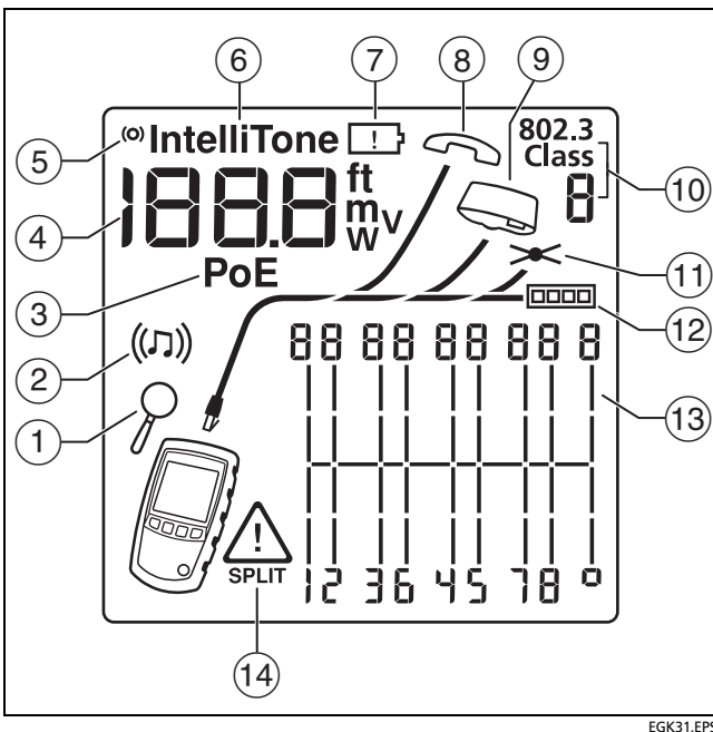
Figure 3. MicroScanner PoE Display Features
