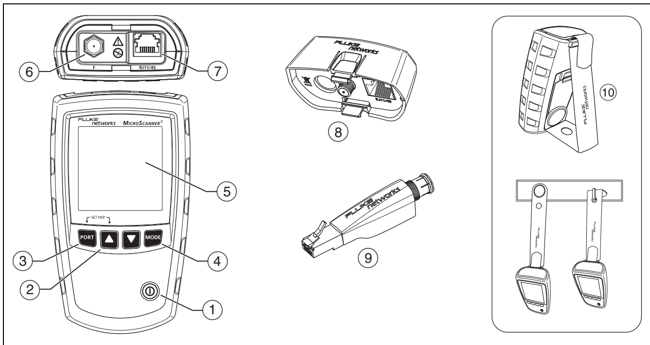
Figure 4. MicroScanner 2 Features
