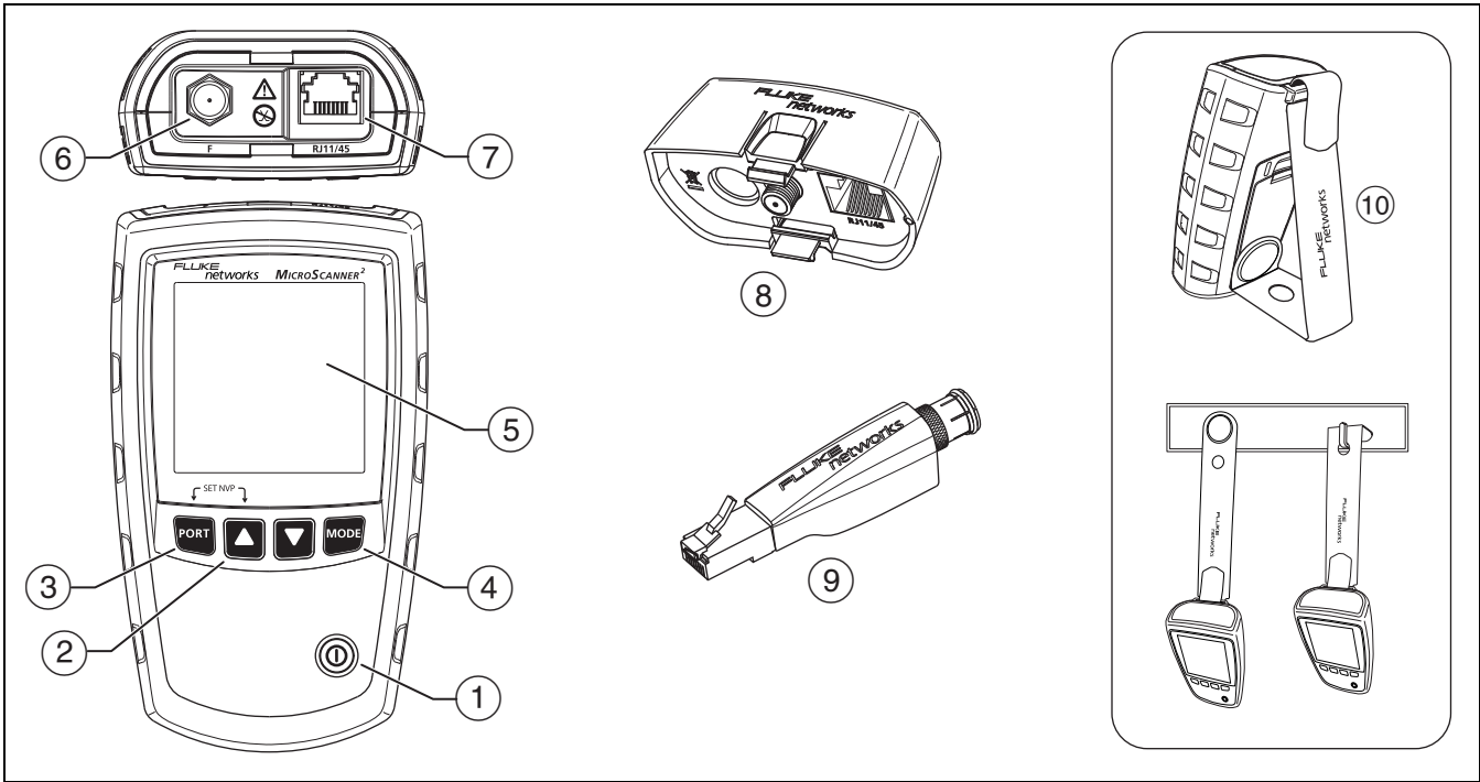
Figure 4. MicroScanner 2 Features
