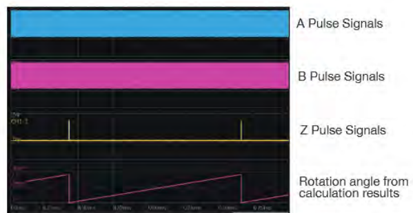
Example of rotary encoder rotation angle waveform
