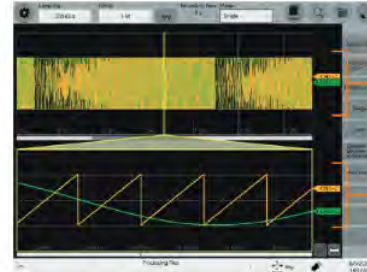
Compressed display of entire recording length
