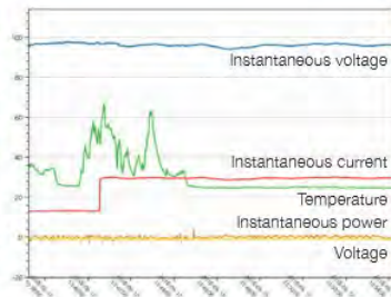
Graph display (up to 32 parameters)
