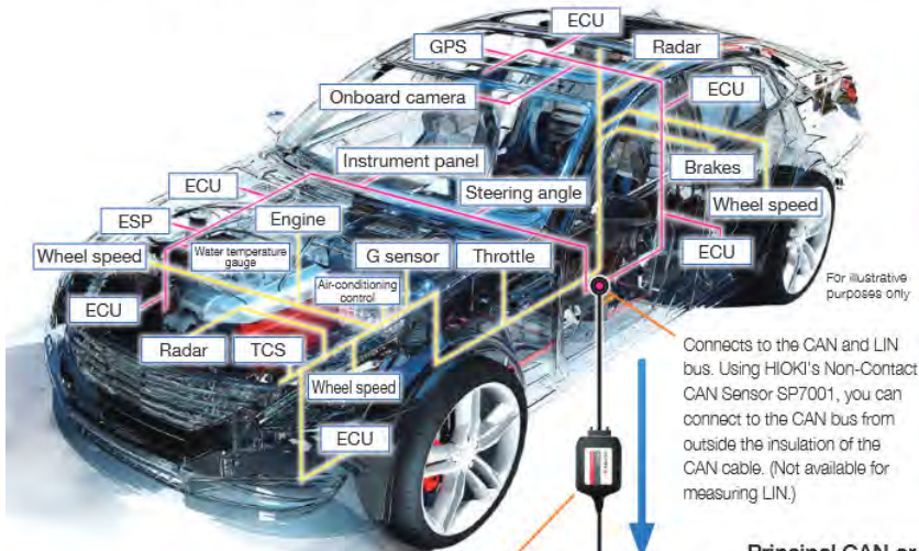
Vector VN1600 interface family
