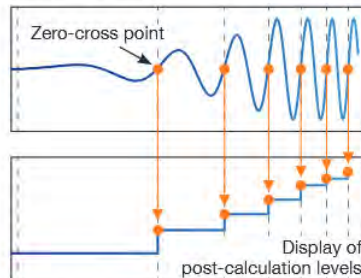
Power calculations based on detected cycles
