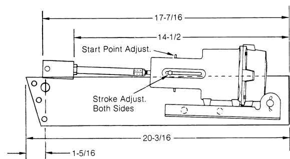
Figure-3 MK-300 Series Dimensions 2 .
