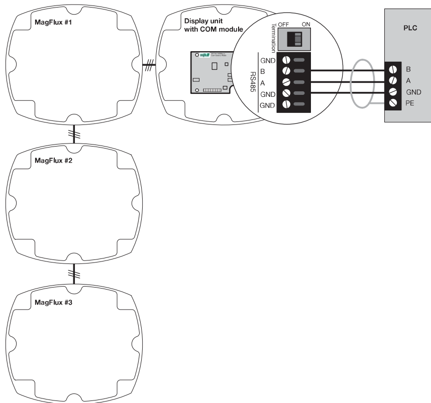
Figure 5. Three Connected Units and One Common Display Unit
