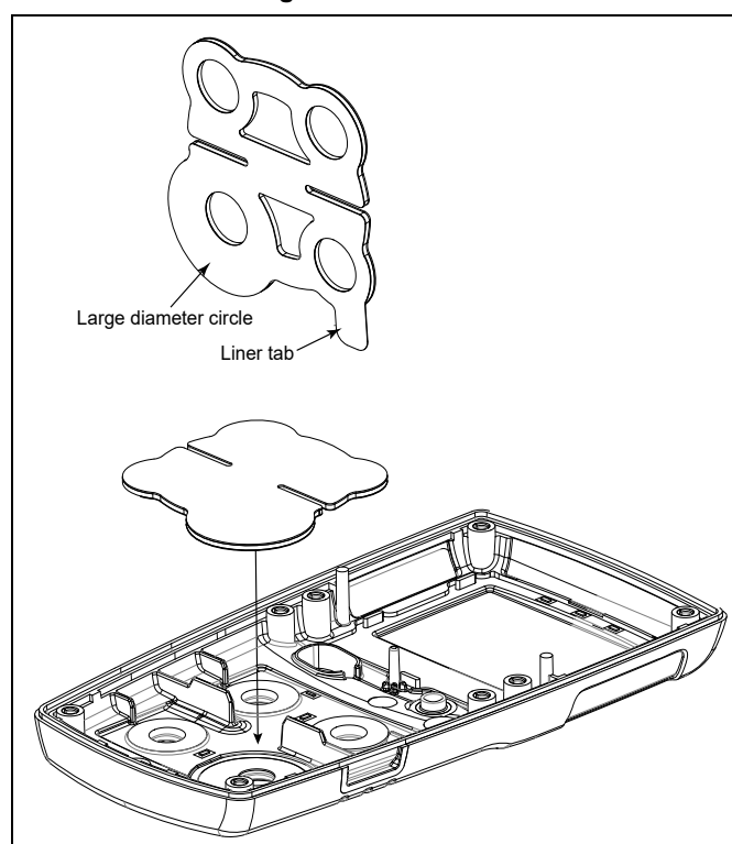
Figure 10. Liner Tab
