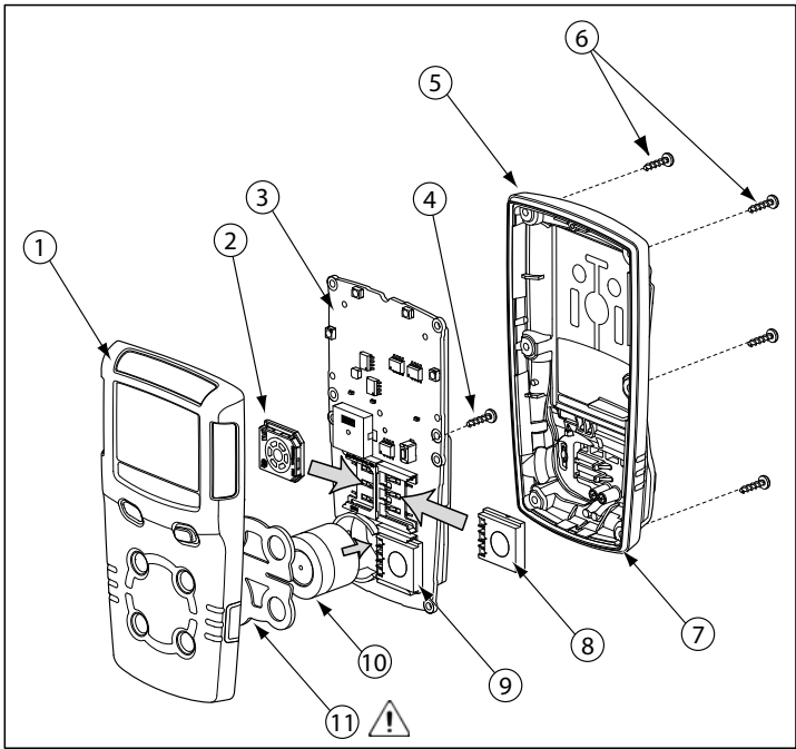
Figure 9. Replacing a Sensor or Sensor Filter
