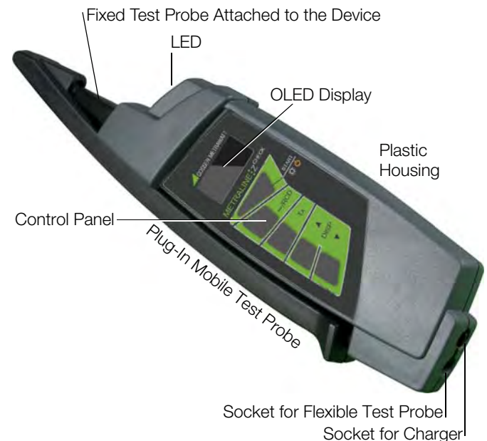
Figure 2.1: Top View
