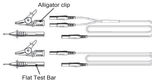
Simplified Measurement Test Leads MODEL 7127A
