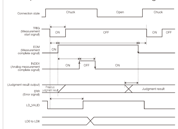
Example of LCR Mode measurement timing
