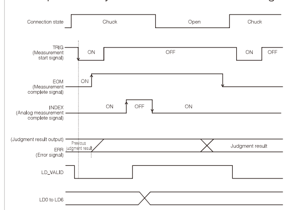
Example of Analyzer Mode measurement timing
