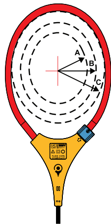
Position sensitivity
